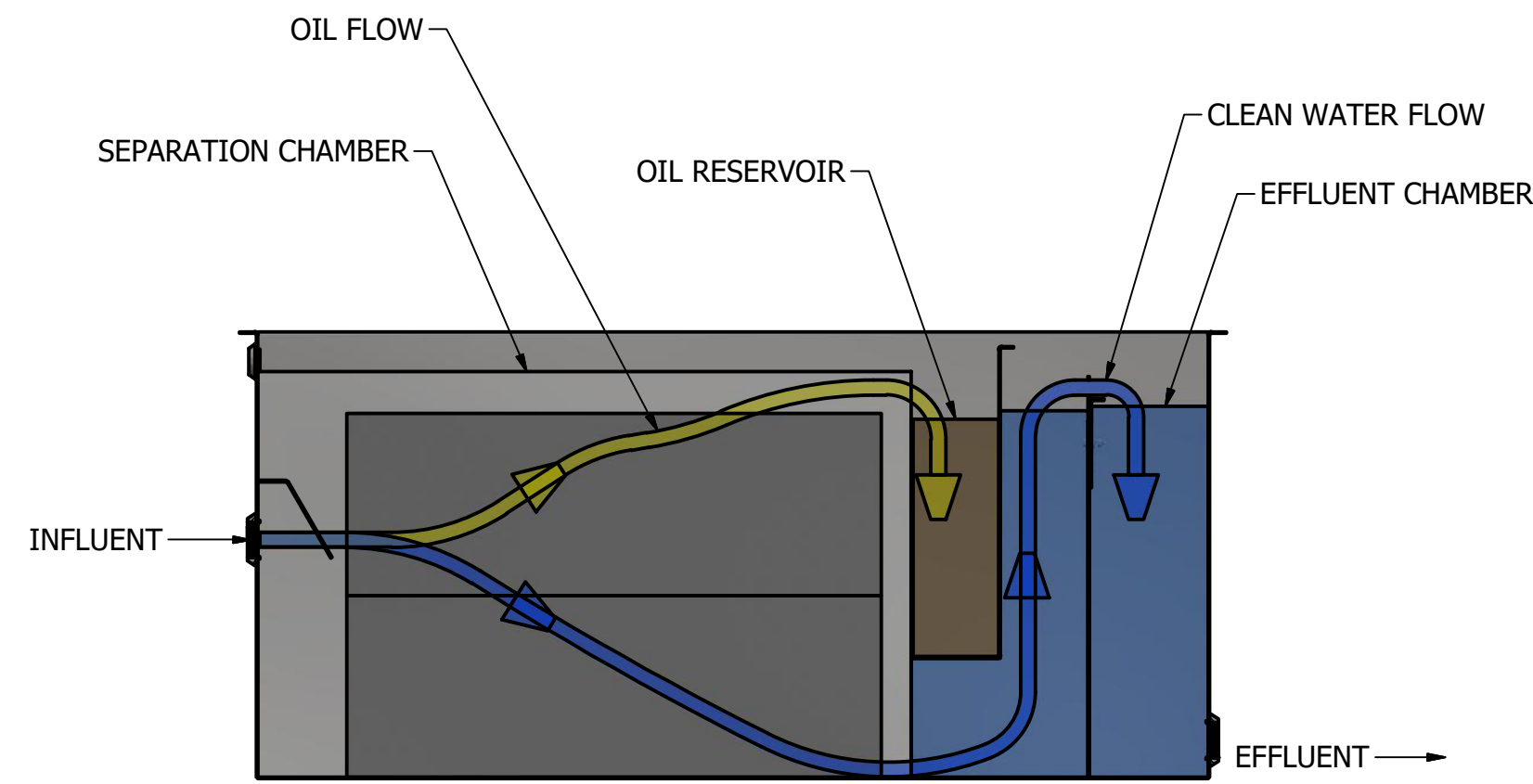
SECTION A-A SCALE 1 / 12
